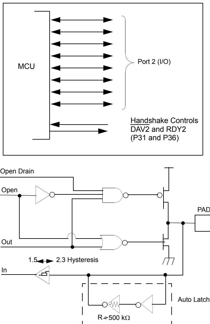
Figure 20. Port 2 Configuration
