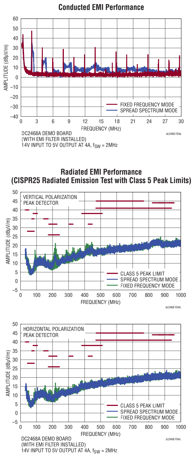
Figure 4. LT8645S Demo Circuit DC2468A EMI Performance (14V Input from VEMI, with EMI Filter, I_{OUT} = 4A )
