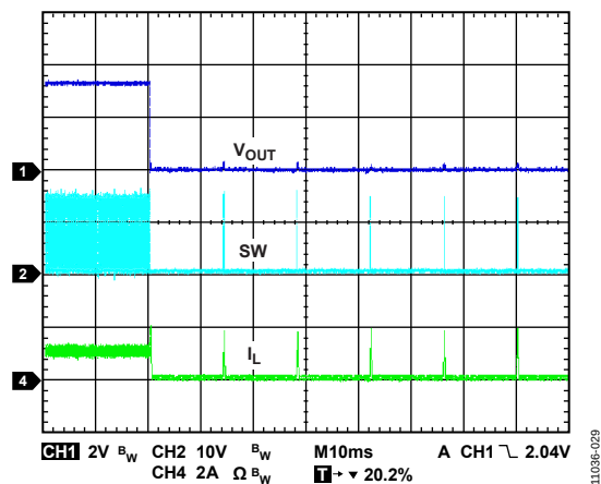
Figure 29. Output Short
