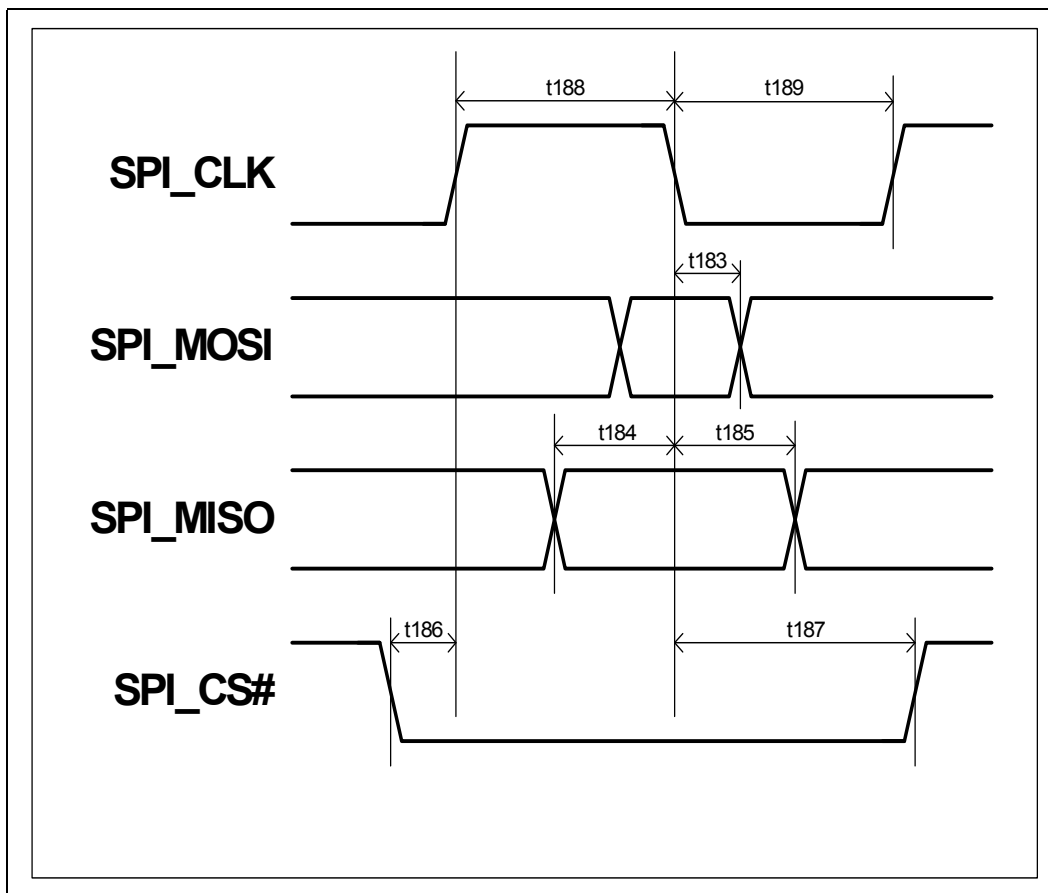
Figure 8-22. SPI Timings
