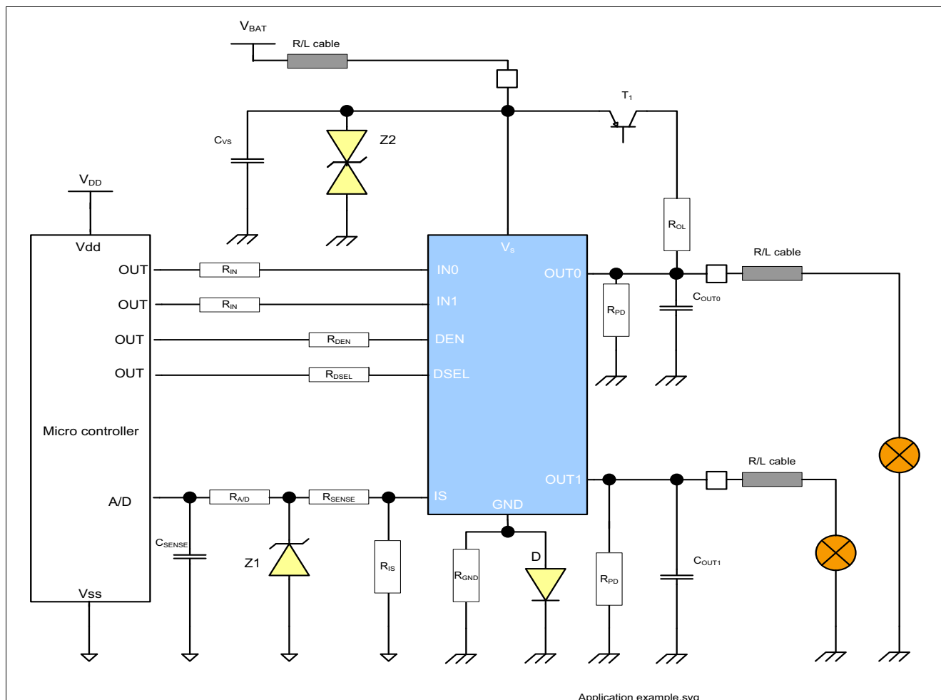
Figure 53 Application Diagram with BTS5045-2EKA
