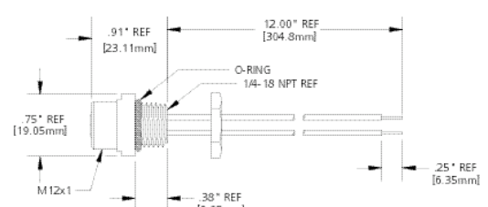
FEMALE RECEPTACLE W/ INTERNAL THREADS AND 1/4" - 18UNF THREADS
