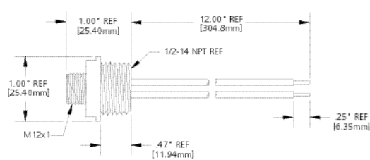
MALE RECEPTACLE W/ EXTERNAL THREADS AND 1/2" - 14UNF THREADS
