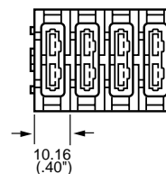
UNASSEMBLED Typical Multiple Mounting (Fuseholders interlocked)
