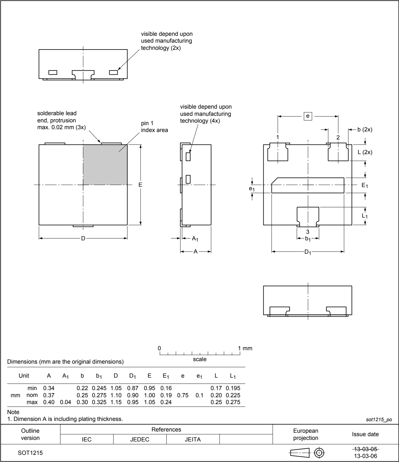
Fig. 11. Package outline DFN1010D-3 (SOT1215)
