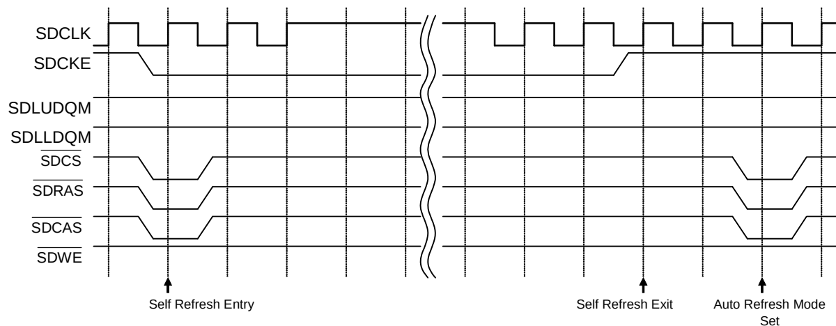
Figure 3.11.7 Self Refresh Cycle Timing
