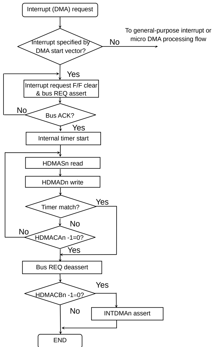
Figure 3.7.9 Overall Flowchart
