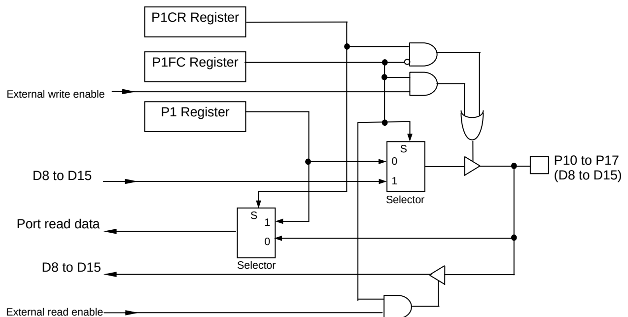
Figure 3.8.1 Port1
