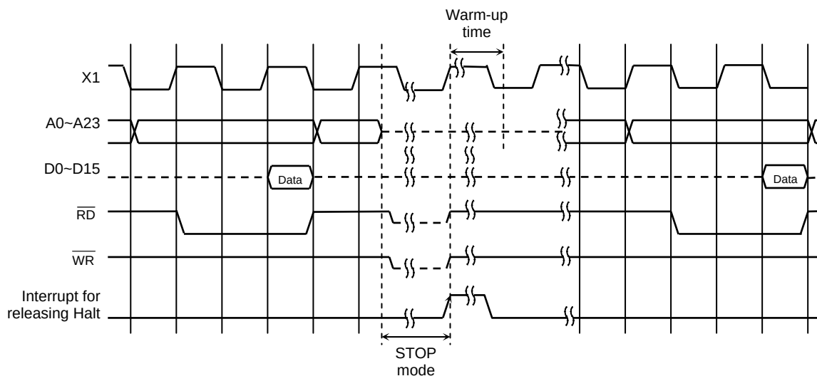
Figure 3.4.9 Timing chart for STOP Mode Halt state cleared by interrupt
