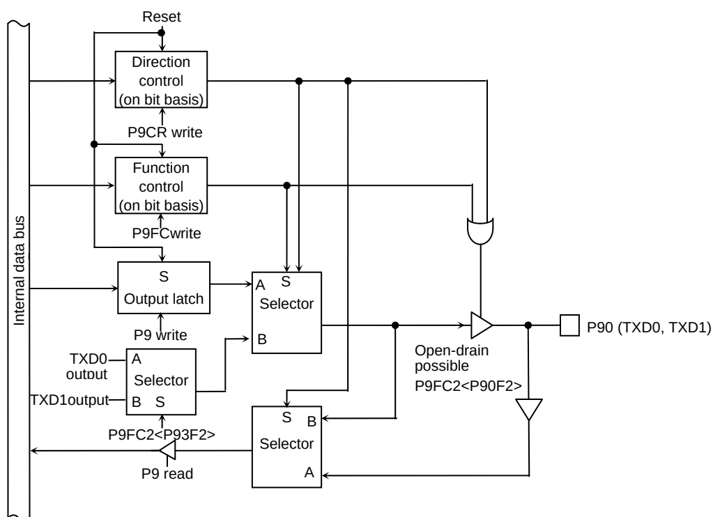
Figure 3.8.14 P90
