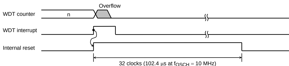
Figure 3.25.3 Reset Mode
