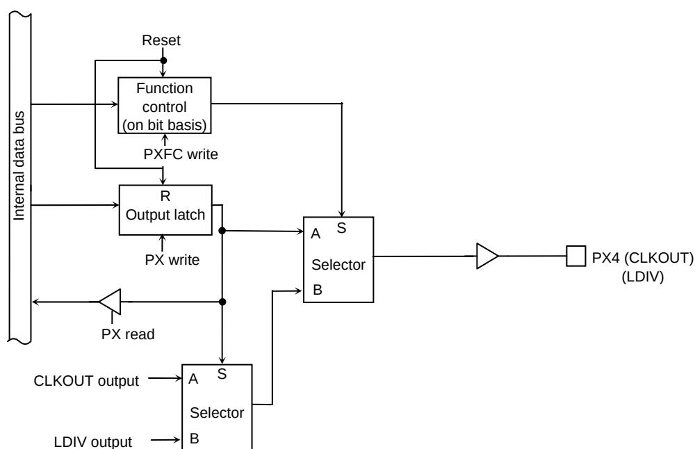
Figure 3.8.56 Port X4
