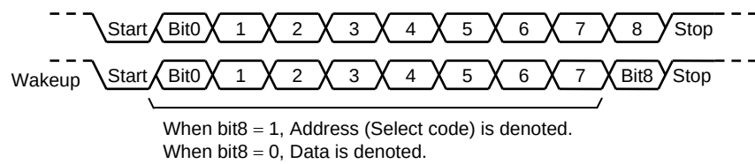
Figure 3.15.1 Data Formats
