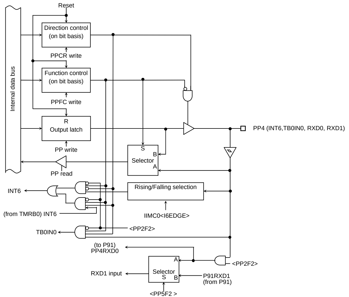
Figure 3.8.45 Port P4
