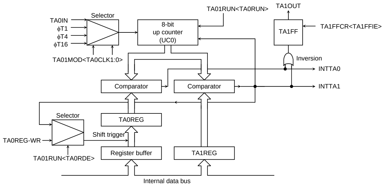
Figure 3.13.20 Block Diagram of 8-Bit PPG Output Mode
