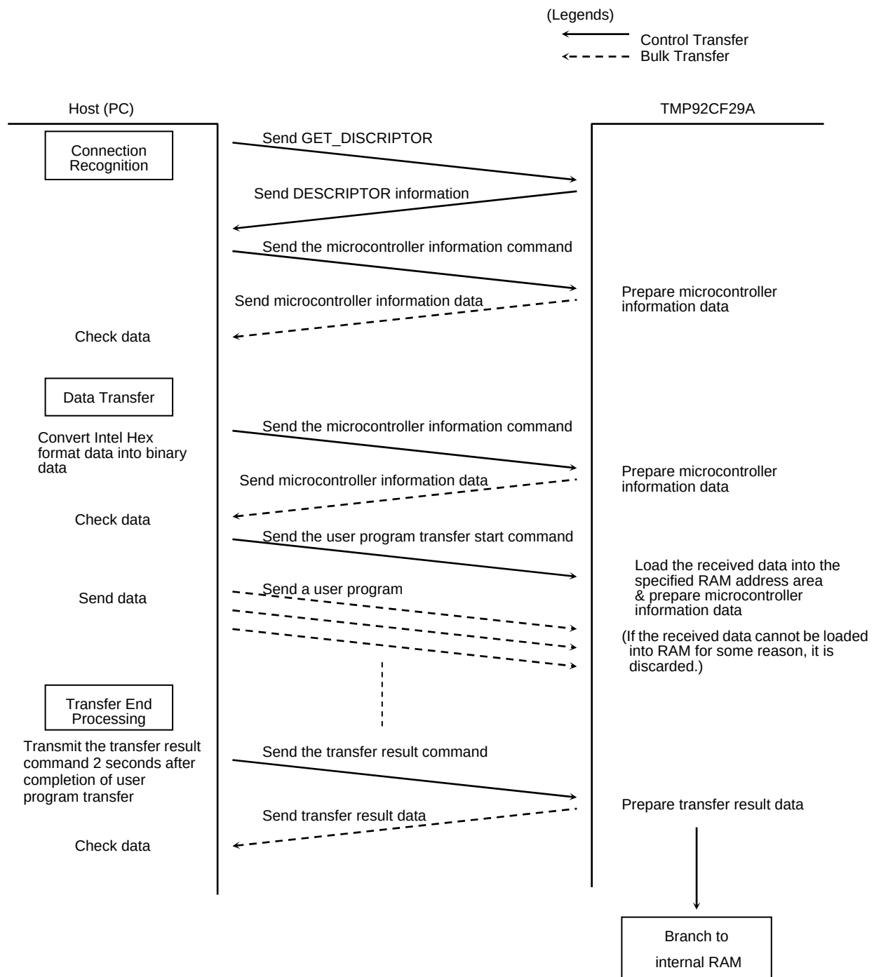
Figure 3.5.6 Overall Flowchart
