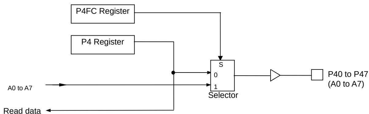
Figure 3.8.3 Port4
