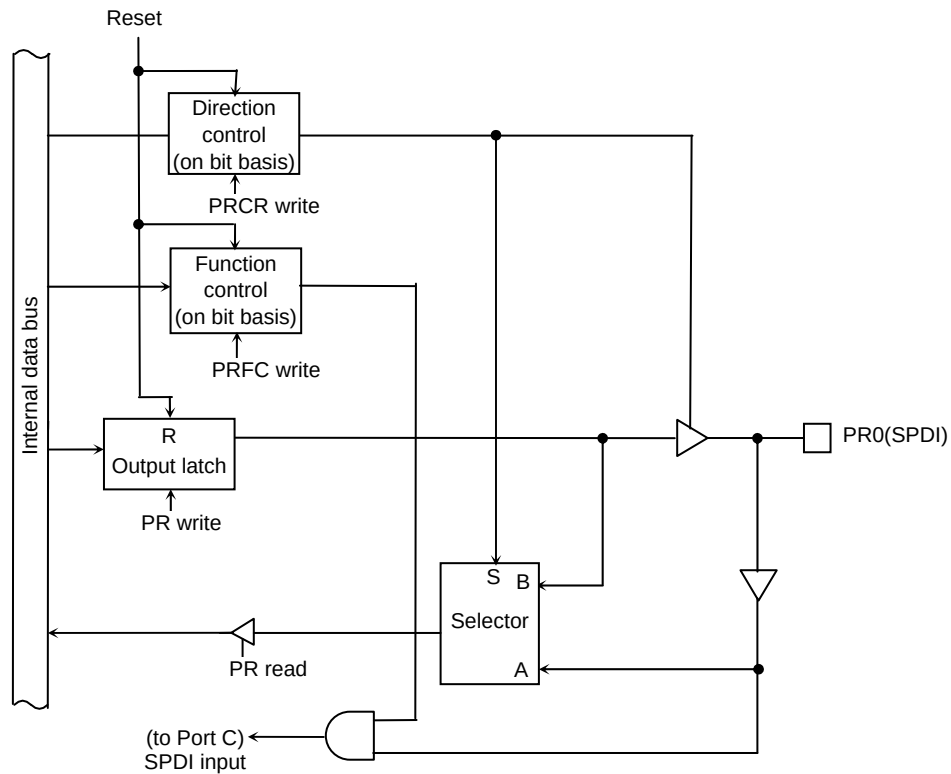
Figure 3.8.49 Port R0
