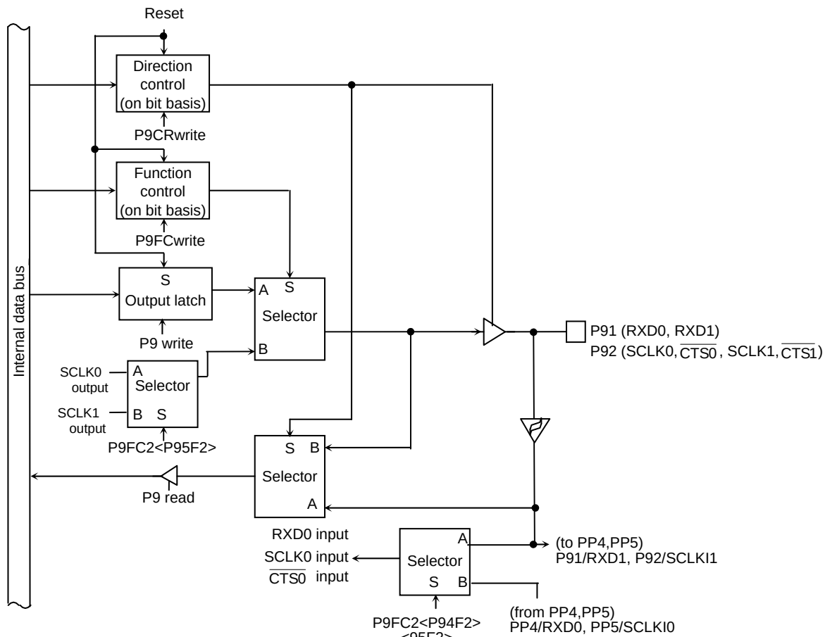
Figure 3.8.15 P91, 92
