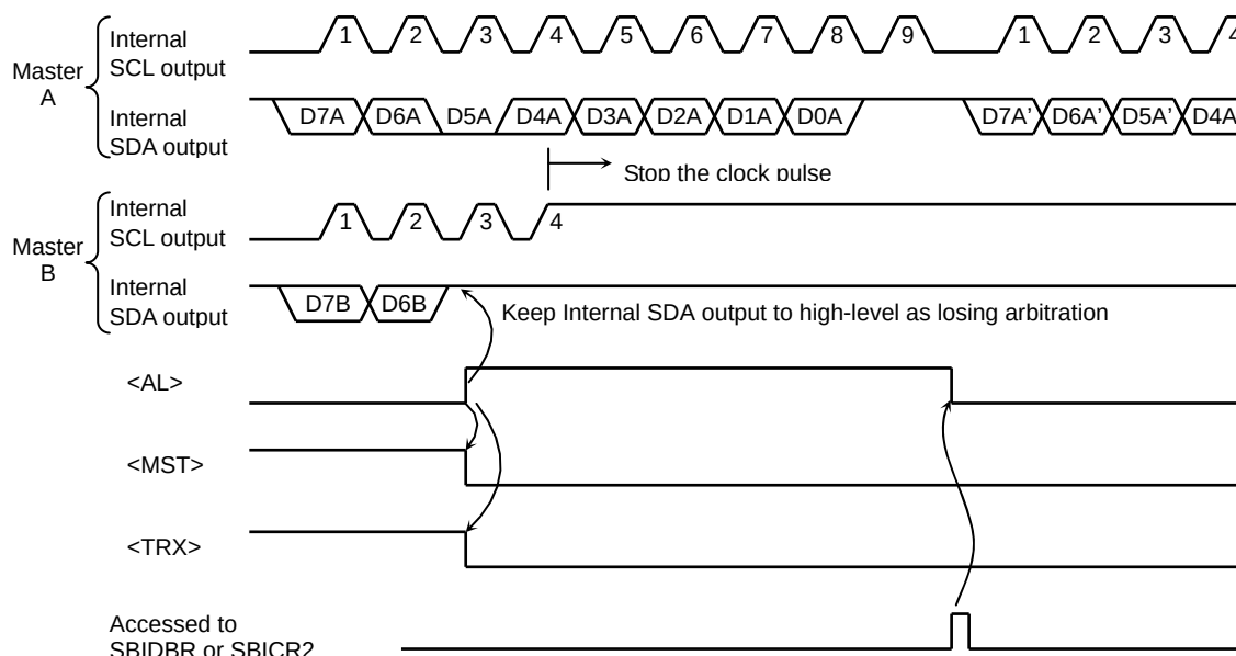
Figure 3.16.13 Example of when TMP92CF29A is a master device B
