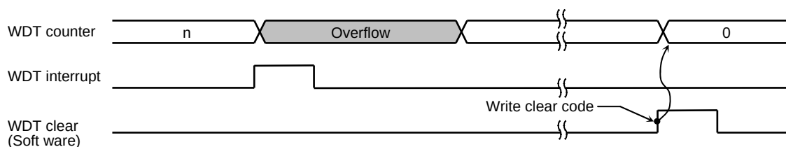
Figure 3.25.2 Normal Mode
