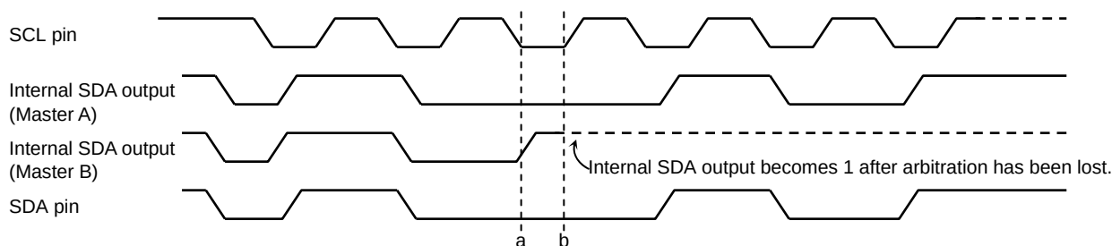
Figure 3.16.12 Arbitration lost
