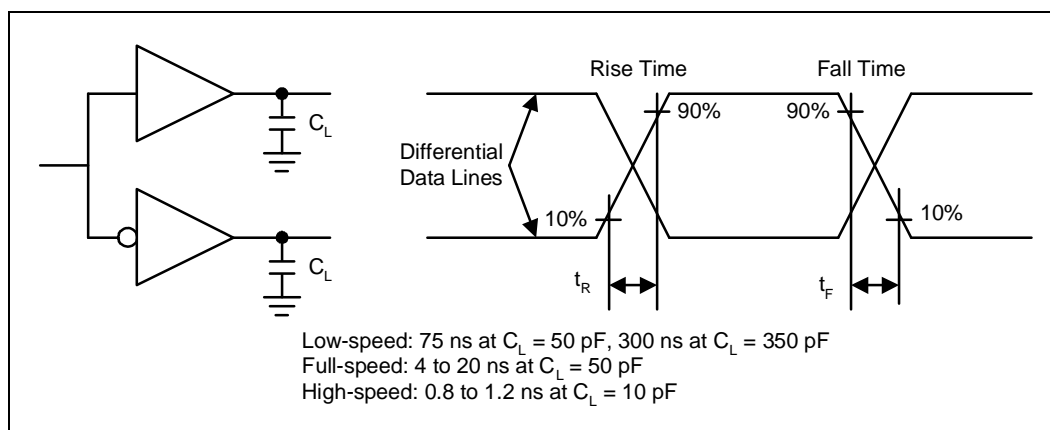
Figure 8-8. USB Jitter
