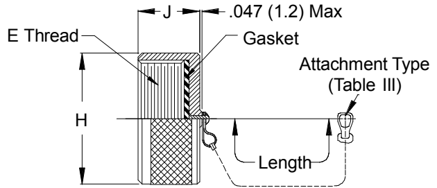
660-005 Receptacle Cover
