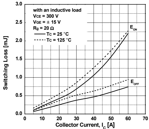
Fig 4. Switching Loss vs. Collector Current - Outer IGBT
