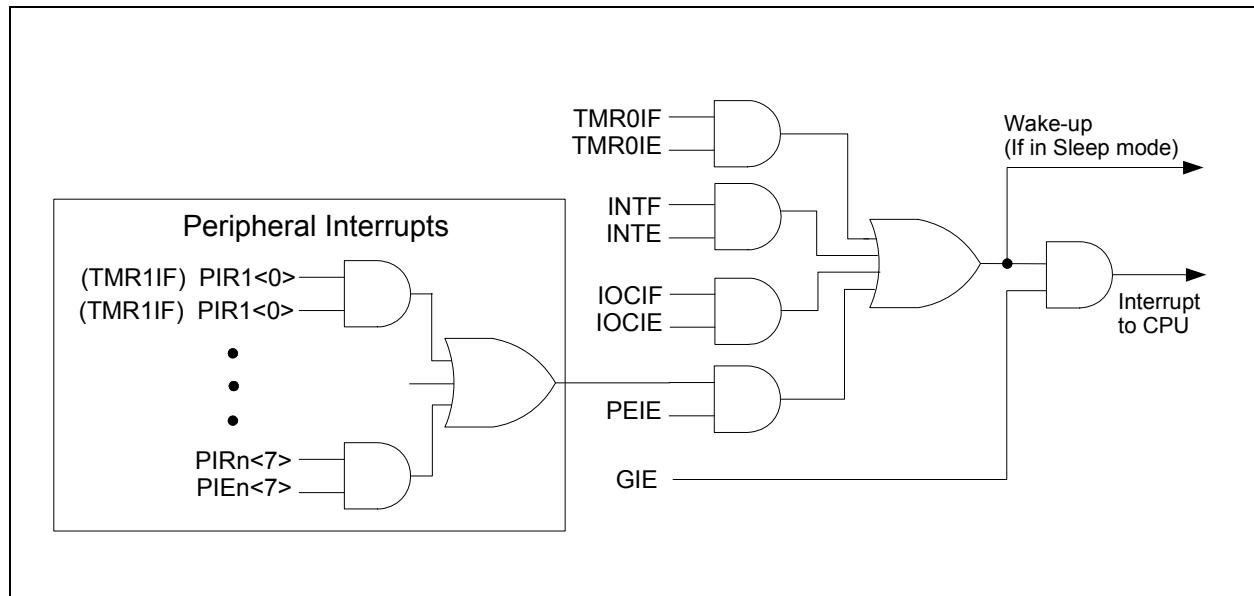
FIGURE 7-1: INTERRUPT LOGIC
