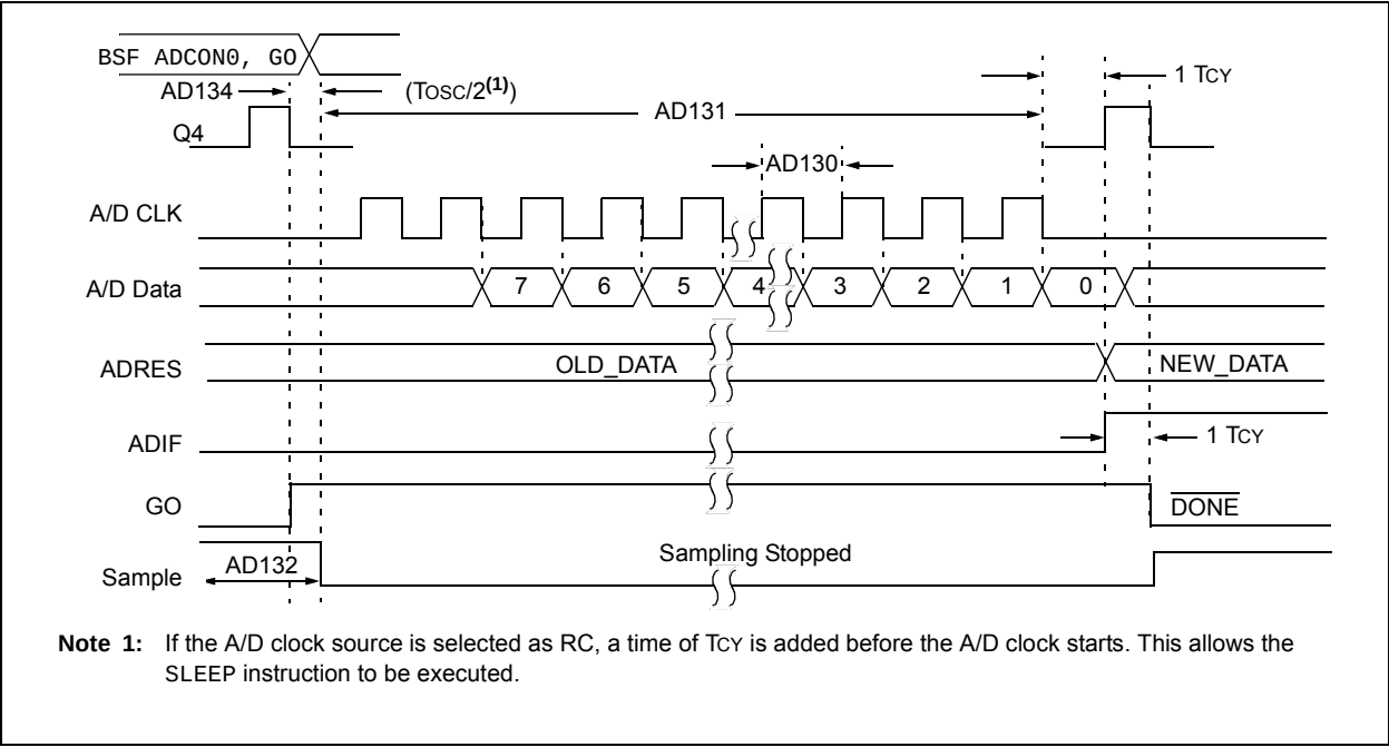
FIGURE 21-10: PIC16LF1902/3 A/D CONVERSION TIMING (NORMAL MODE)
