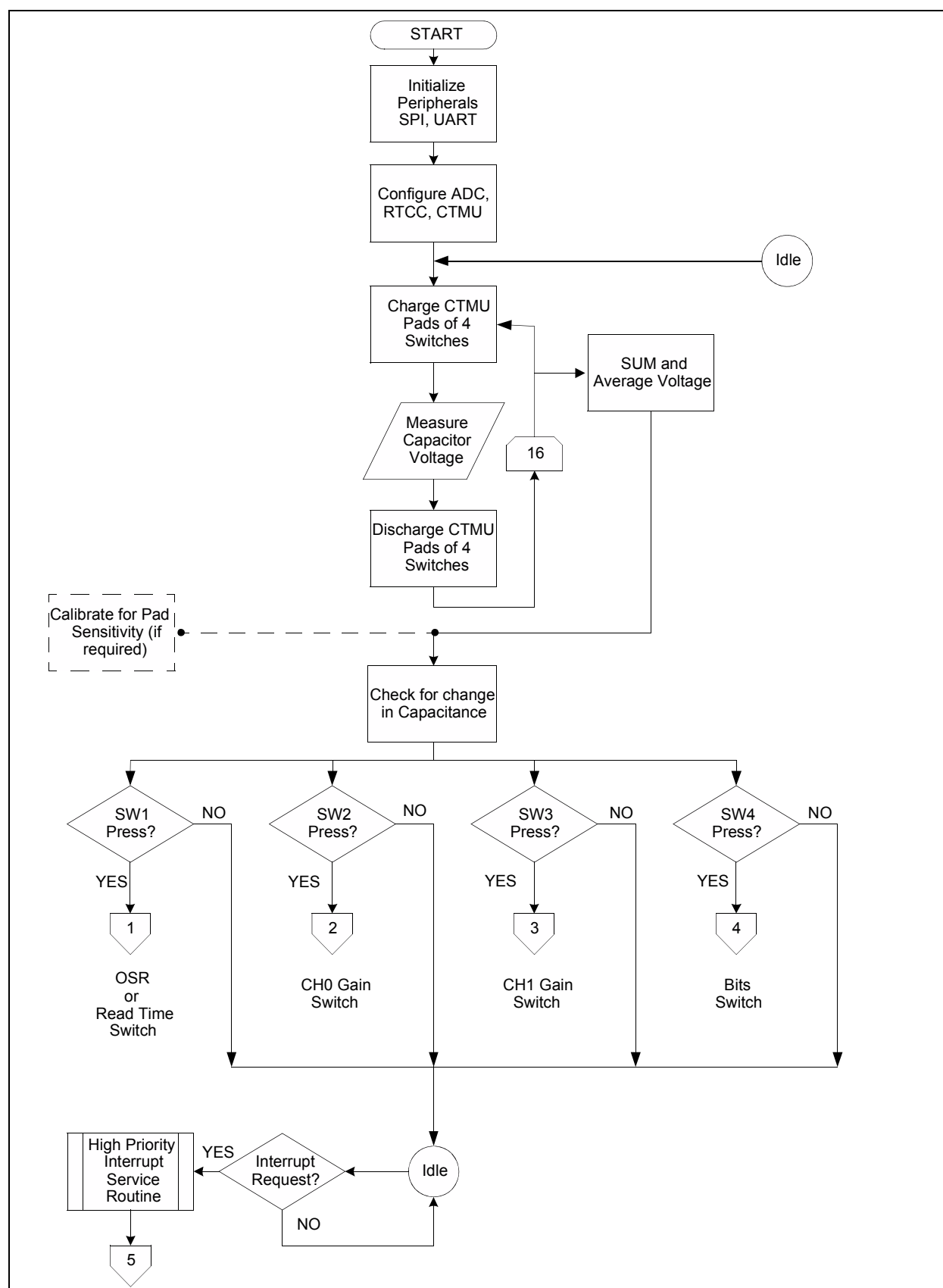
FIGURE 4-1: Main Routine
