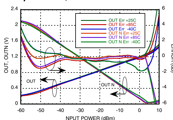
Output Voltage & Error vs. Input Power, F_{in} = 2700 MHz
