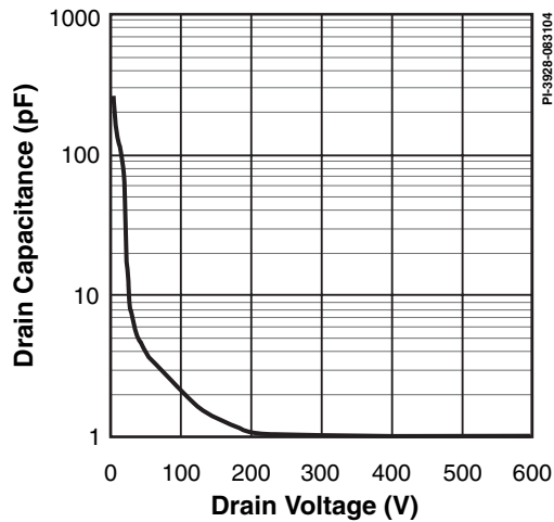
Figure 16. C_{DSS} vs. Drain Voltage.
