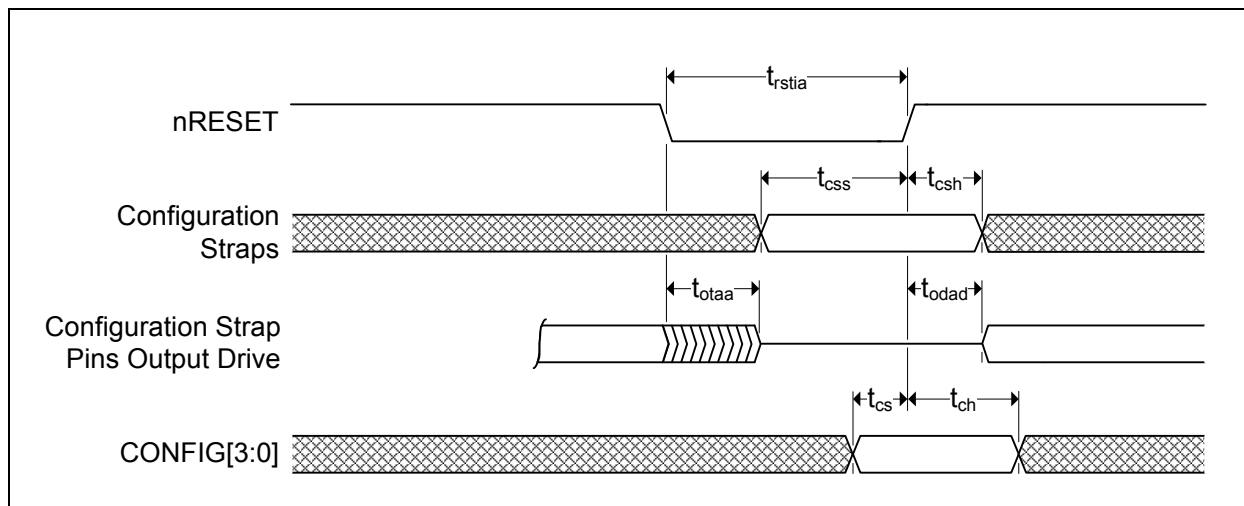
FIGURE 5-4: RESET TIMING
