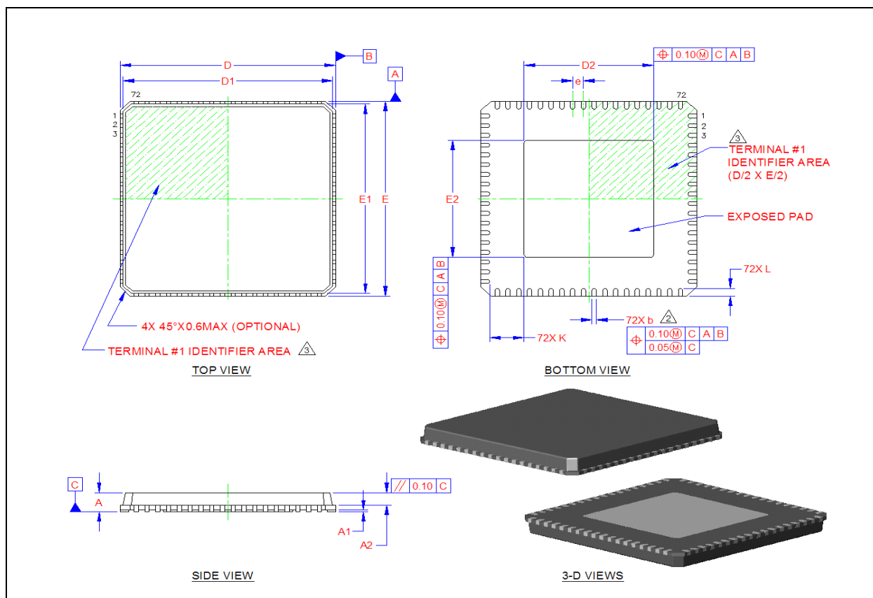
FIGURE 6-1: 72-QFN PACKAGE
