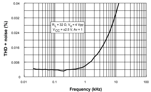
Figure 8. THD + noise vs. frequency ( R_L = 32\text{ }\Omega , V_O = 4\text{ Vpp} , V_{CC} = \pm 2.5\text{ V} )
