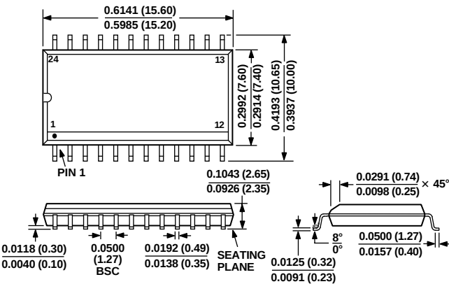
24-Lead SOIC Package (R-24)
