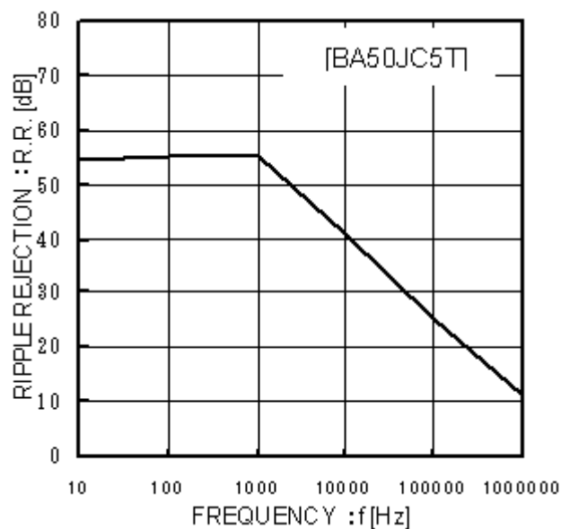
Fig.8 Ripple Rejection
