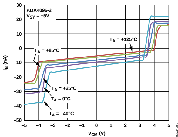
Figure 22. Input Bias Current vs. V CM and Temperature
