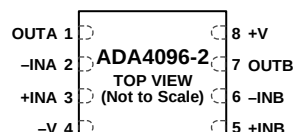
Figure 5. 8-Lead LFCSP (CP-8-10), ADA4096-2
