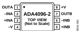
Figure 4. 8-Lead, MSOP (RM-8), ADA4096-2
