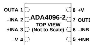
Figure 1. 8-Lead, MSOP (RM-8), ADA4096-2
