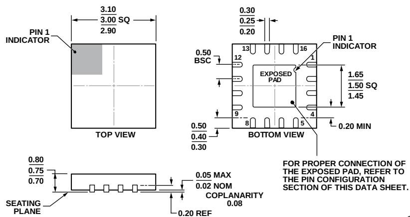
Figure 57. 16-Lead Lead Frame Chip Scale Package [LFCSF_WQ] 3 mm × 3 mm Body, Very Very Thin Quad (CP-16-27)
