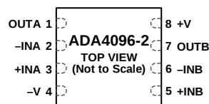
Figure 5. 8-Lead LFCSP (CP-8-10), ADA4096-2
