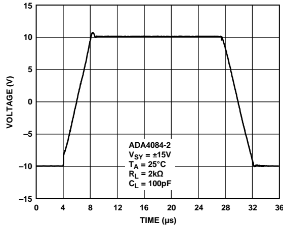
Figure 68. Large Signal Transient Response
