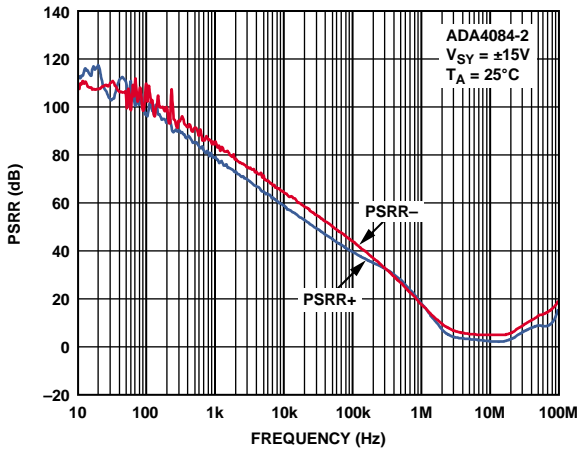
Figure 66. PSRR vs. Frequency
