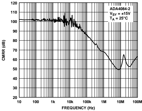
Figure 67. CMRR vs. Frequency
