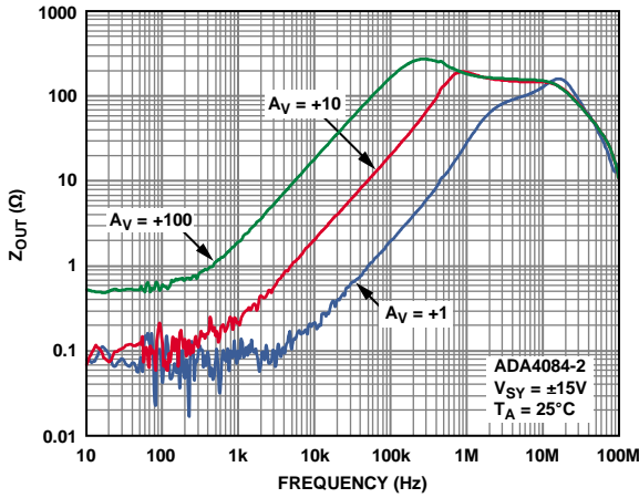
Figure 65. Output Impedance vs. Frequency
