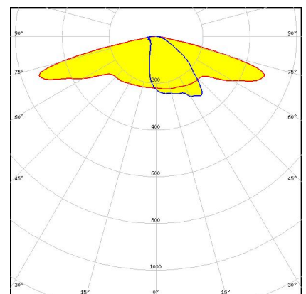
CS15055_STRADA-IP-2X6-DWC-90-PC
