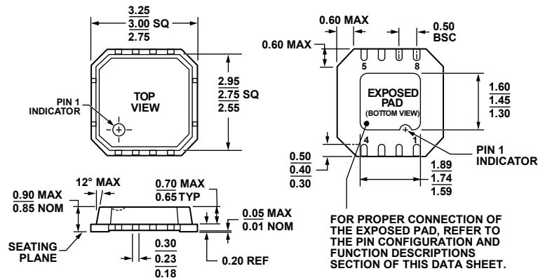
Figure 64. 8-Lead Lead Frame Chip Scale Package [LFCSP_VD]
