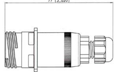
Backshell used with PCB Receptacle back-termination - (Type 2) Sealed version – IP67
