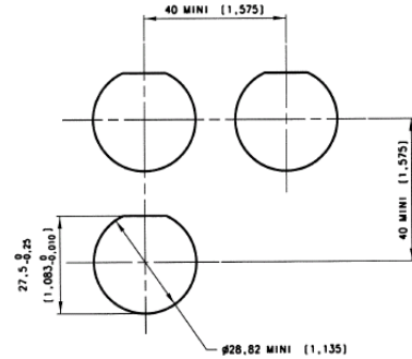
Panel Drilling
