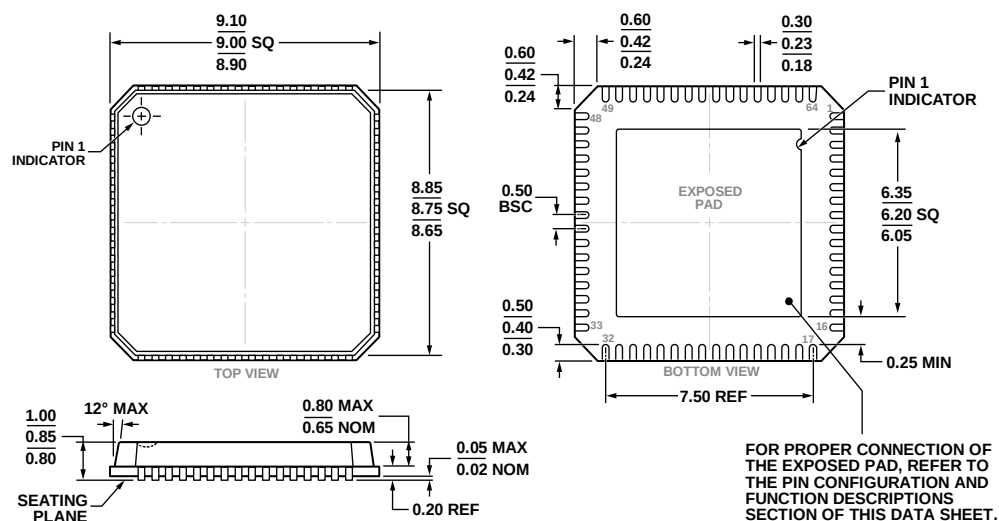
Figure 62. 64-Lead Lead Frame Chip Scale Package [LFCSP_VQ] 9 mm x 9 mm Body, Very Thin Quad (CP-64-4)
