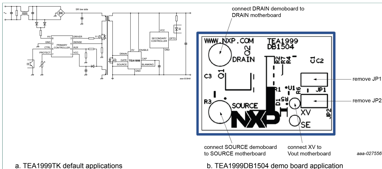
Figure 4. Connections for low-side SR
