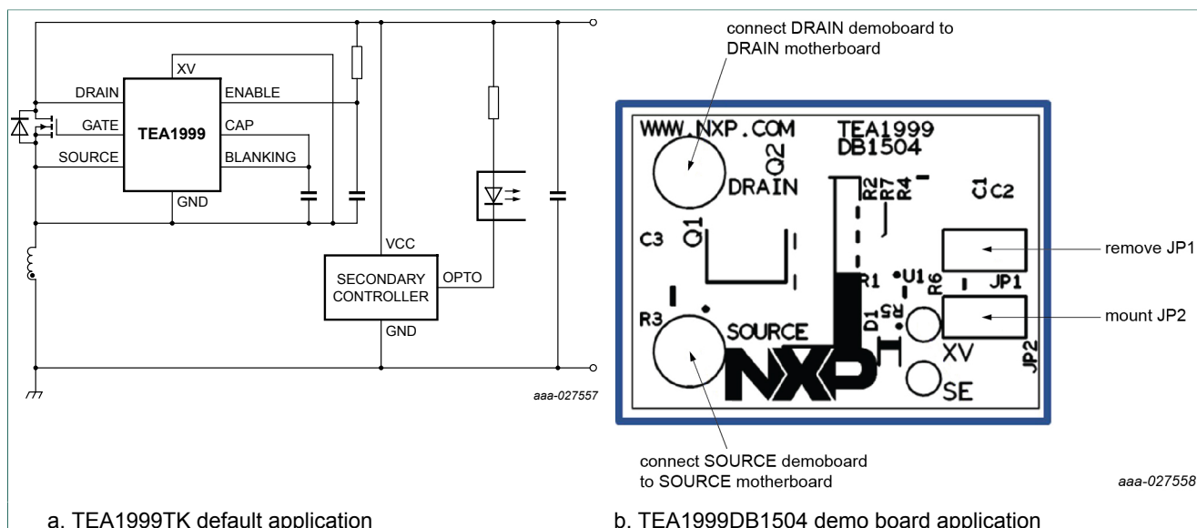
Figure 5. Connections for high-side SR with self-supply
