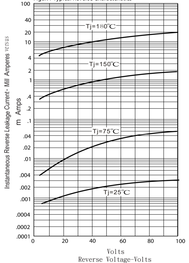
Figur.4-Typical Reverse Characteristics
