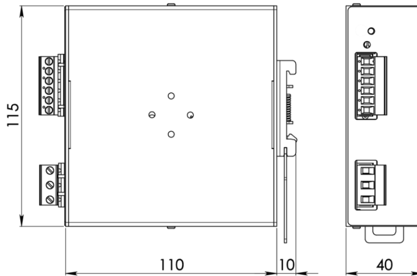
Figure 1. Mechanical Drawing
