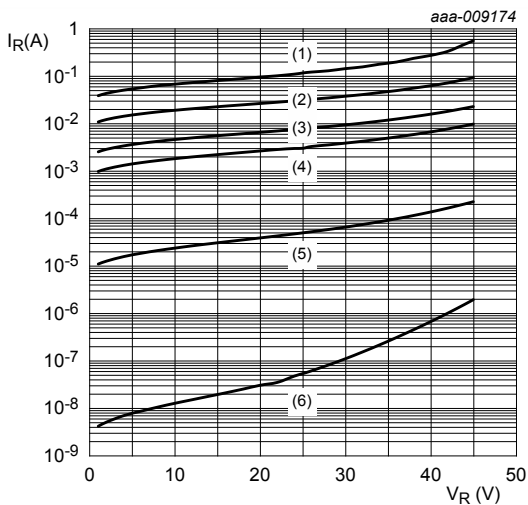
pulsed conditions (1) T_j = 150\text{ }^{\circ}\text{C} (2) T_j = 125\text{ }^{\circ}\text{C} (3) T_j = 100\text{ }^{\circ}\text{C} (4) T_j = 85\text{ }^{\circ}\text{C} (5) T_j = 25\text{ }^{\circ}\text{C} (6) T_j = -40\text{ }^{\circ}\text{C}
