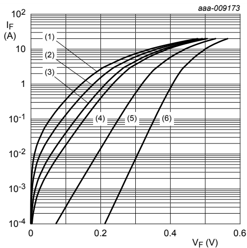
pulsed condition (1) T_j = 150\text{ }^{\circ}\text{C} (2) T_j = 125\text{ }^{\circ}\text{C} (3) T_j = 100\text{ }^{\circ}\text{C} (4) T_j = 85\text{ }^{\circ}\text{C} (5) T_j = 25\text{ }^{\circ}\text{C} (6) T_j = -40\text{ }^{\circ}\text{C}
