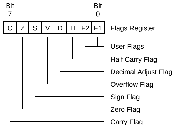
Figure 58. Flags Register
