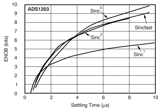
Figure 28. Effective Number of Bits vs Settling Time (ADS1203)
