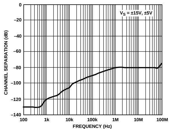
Figure 29. Channel Separation
