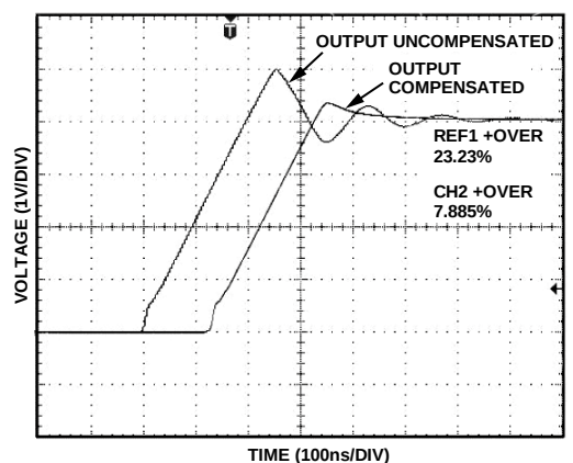
Figure 30. Transient Output Response
