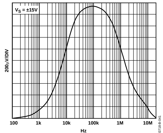
Figure 39. Band-Pass Response
