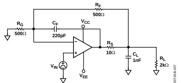
Figure 35. Recommended Capacitive Load Circuit
