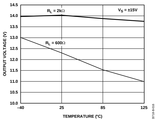
Figure 14. Output Voltage High vs. Temperature
