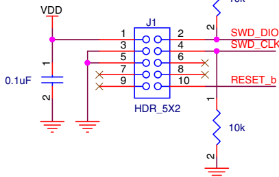
Figure 23. SWD debug interface
