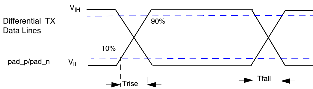
Figure 32. Rise/fall time
