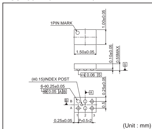
VCSP50L1 (BD2204GUL)
