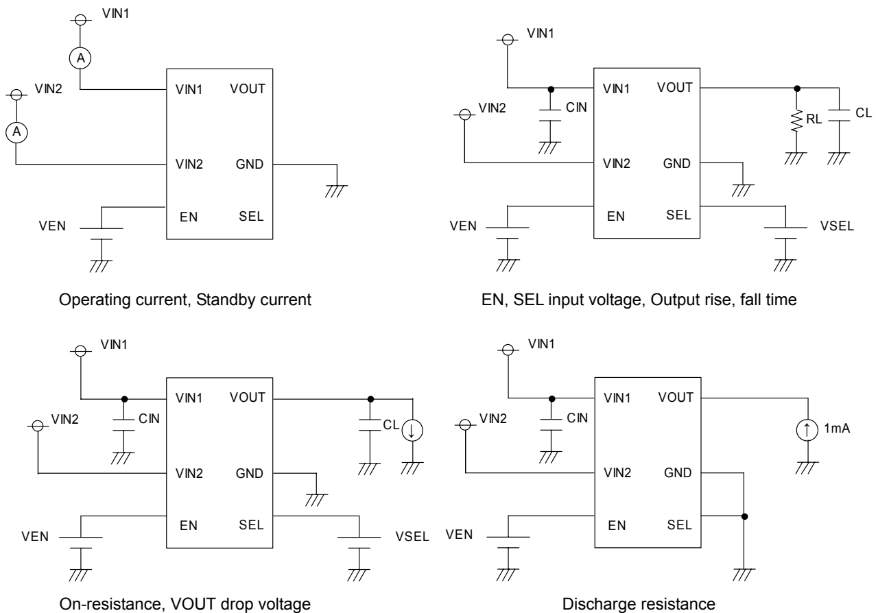
Figure 5. Measurement circuit
