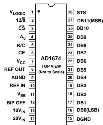
PIN CONFIGURATION
