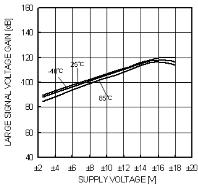
Figure 17. Large Signal Voltage Gain - Supply Voltage ( R_L=2k\Omega )
