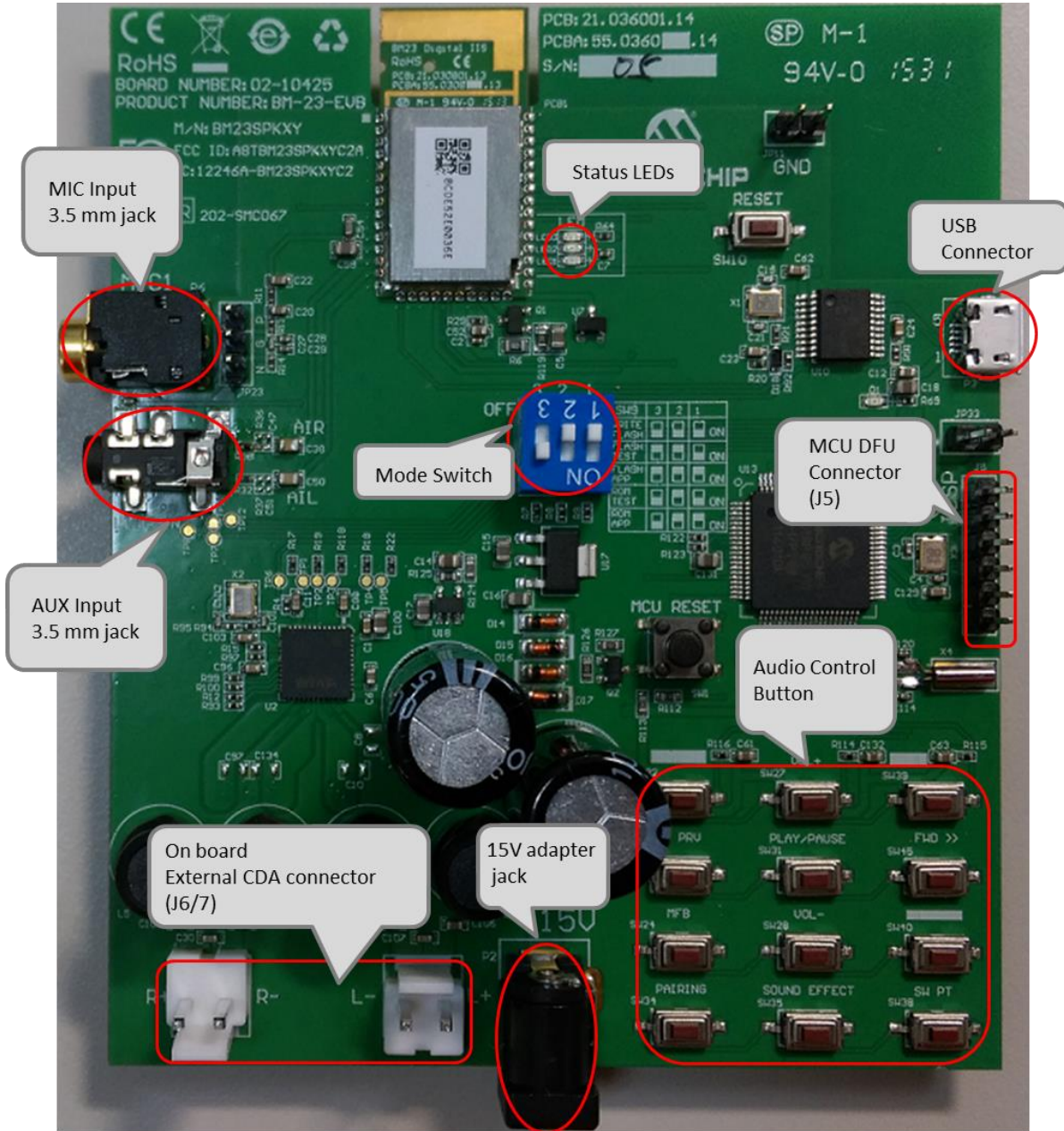
FIGURE 1-1: BM23 EVALUATION BOARD
