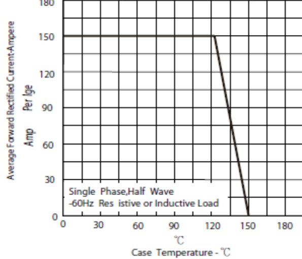
Figure.2-Forward Derating Curve
