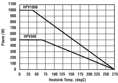
Derating Curve
