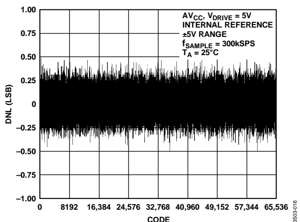
Figure 14. Typical DNL, \pm 5\text{ V} Range
