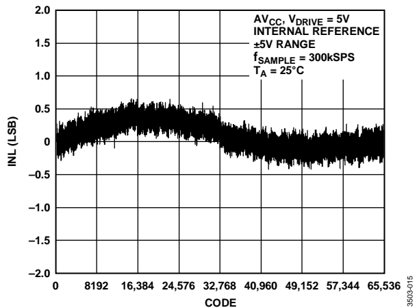
Figure 13. Typical INL, \pm 5\text{ V} Range
