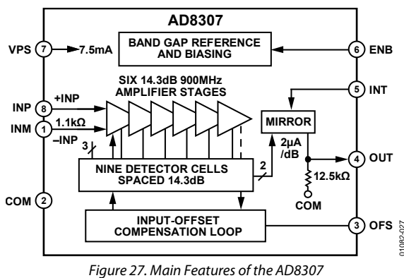
Figure 27. Main Features of the AD8307
